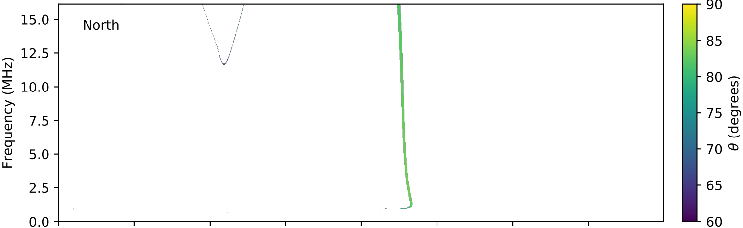
expres_cassini_jupiter_io_isaac_lossc-wid1deg_3kev_20030323_v01.cdf
