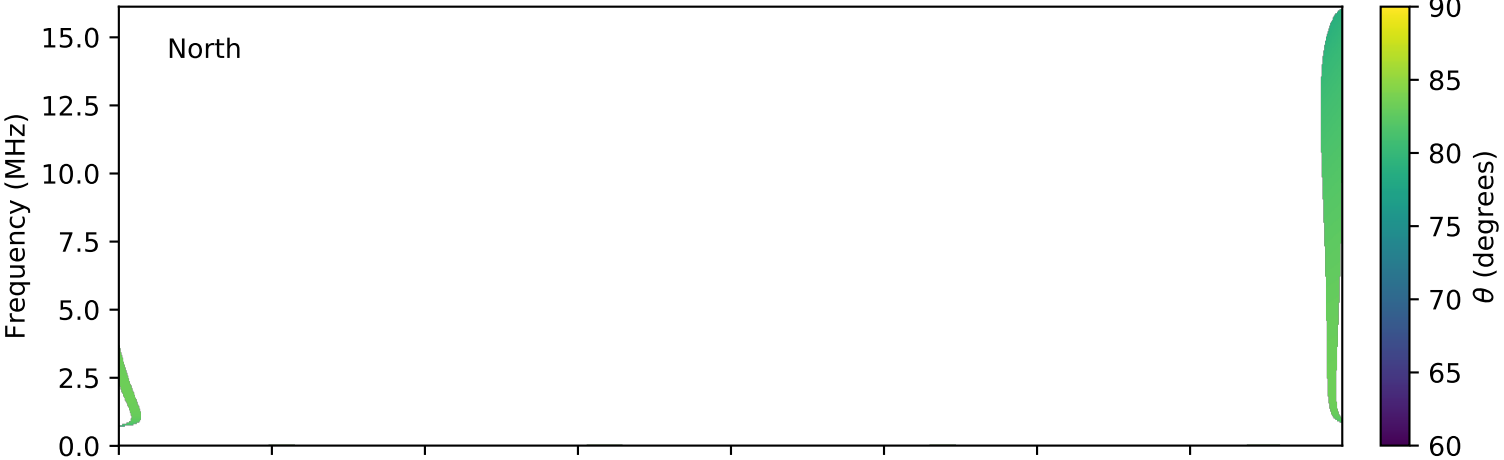
expres_cassini_jupiter_io_isaac_lossc-wid1deg_3kev_20030320_v01.cdf
