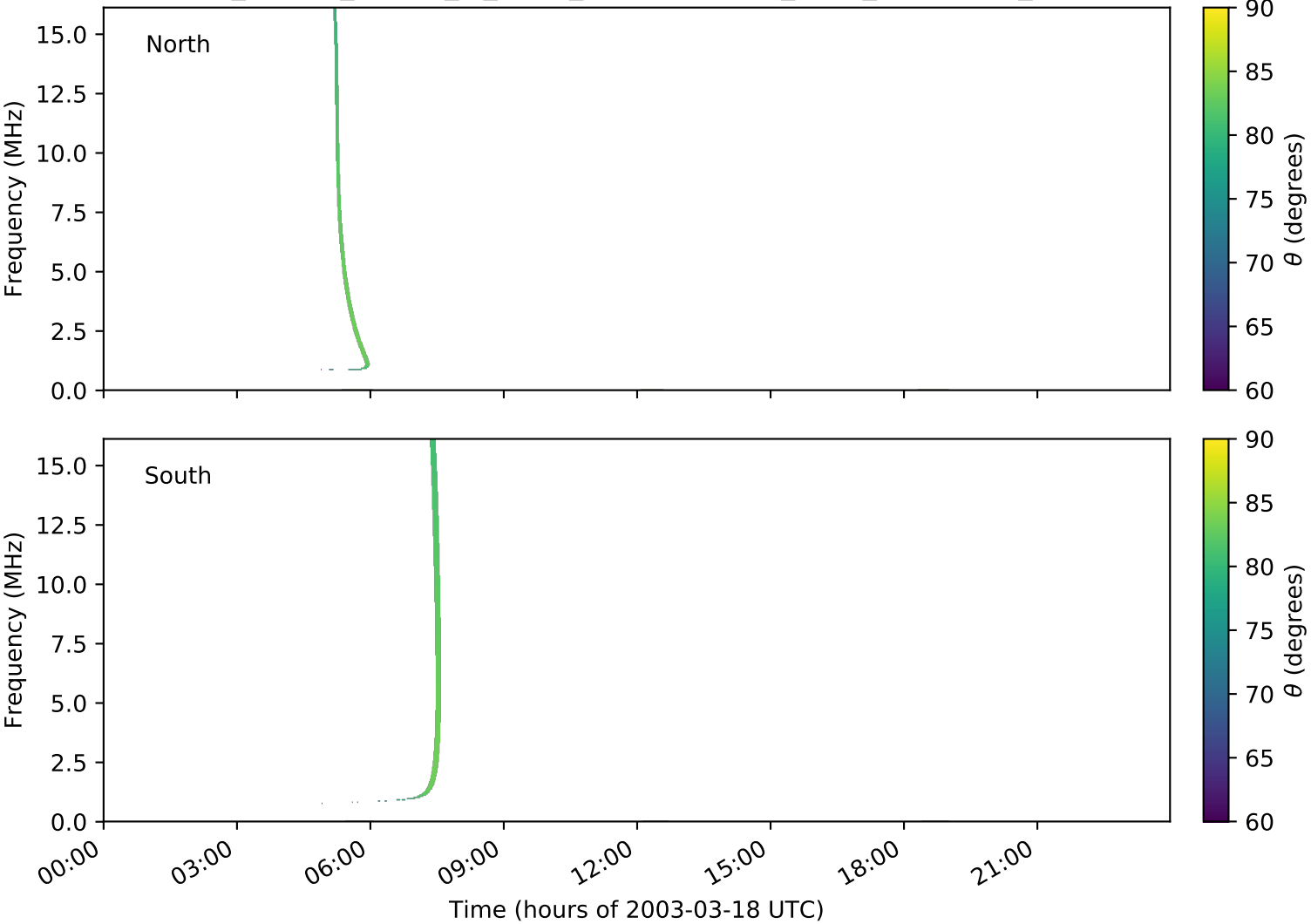
expres_cassini_jupiter_io_isaac_lossc-wid1deg_3kev_20030318_v01.cdf
