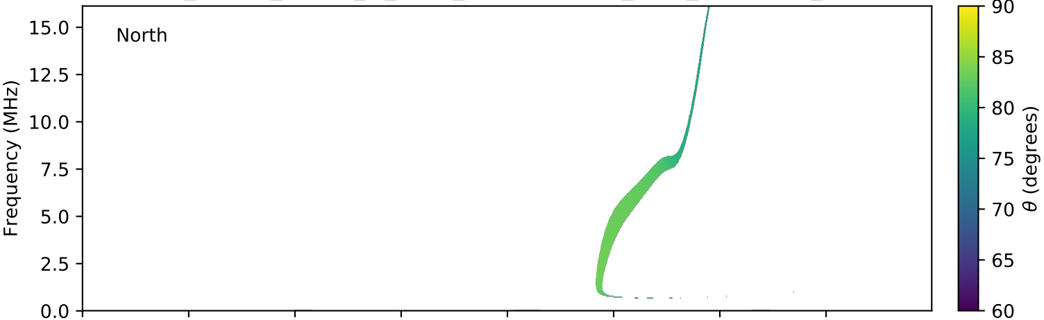
expres_cassini_jupiter_io_isaac_lossc-wid1deg_3kev_20030308_v01.cdf
