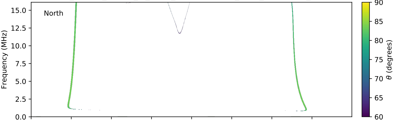
expres_cassini_jupiter_io_isaac_lossc-wid1deg_3kev_20030305_v01.cdf
