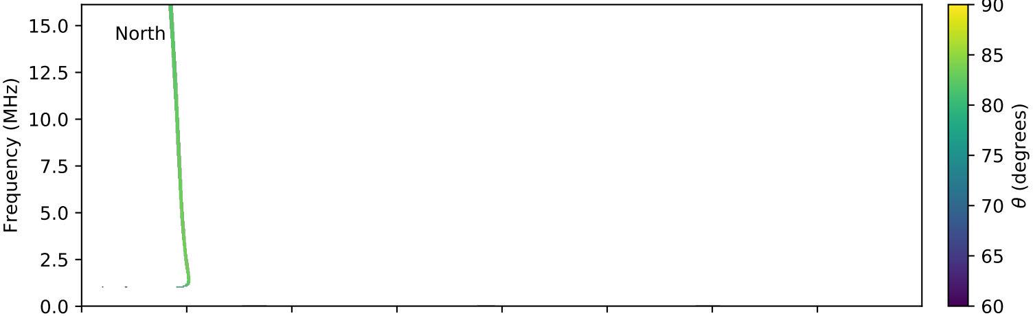
expres_cassini_jupiter_io_isaac_lossc-wid1deg_3kev_20030304_v01.cdf
