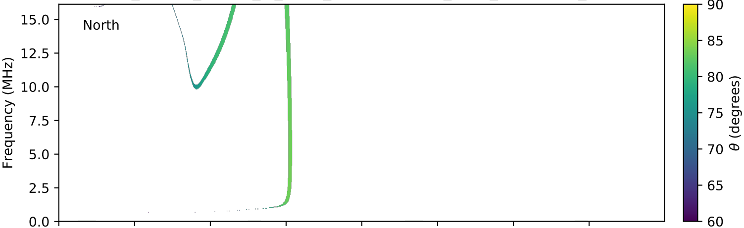
expres_cassini_jupiter_io_isaac_lossc-wid1deg_3kev_20030302_v01.cdf
