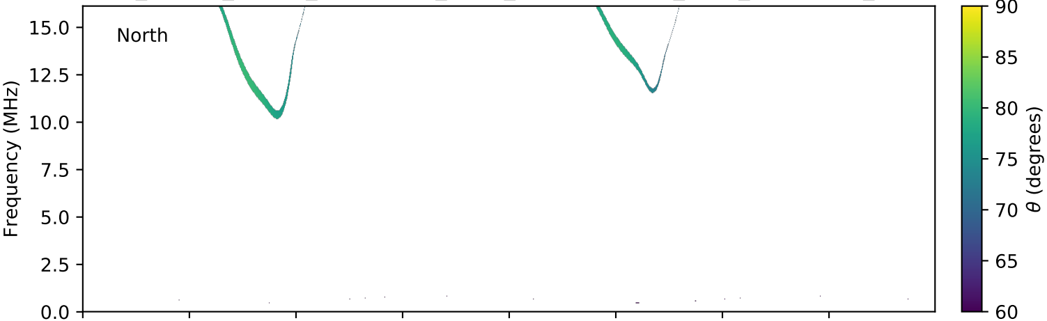
expres_cassini_jupiter_ganymede_isaac_lossc-wid1deg_3kev_20030330_v01.cdf
