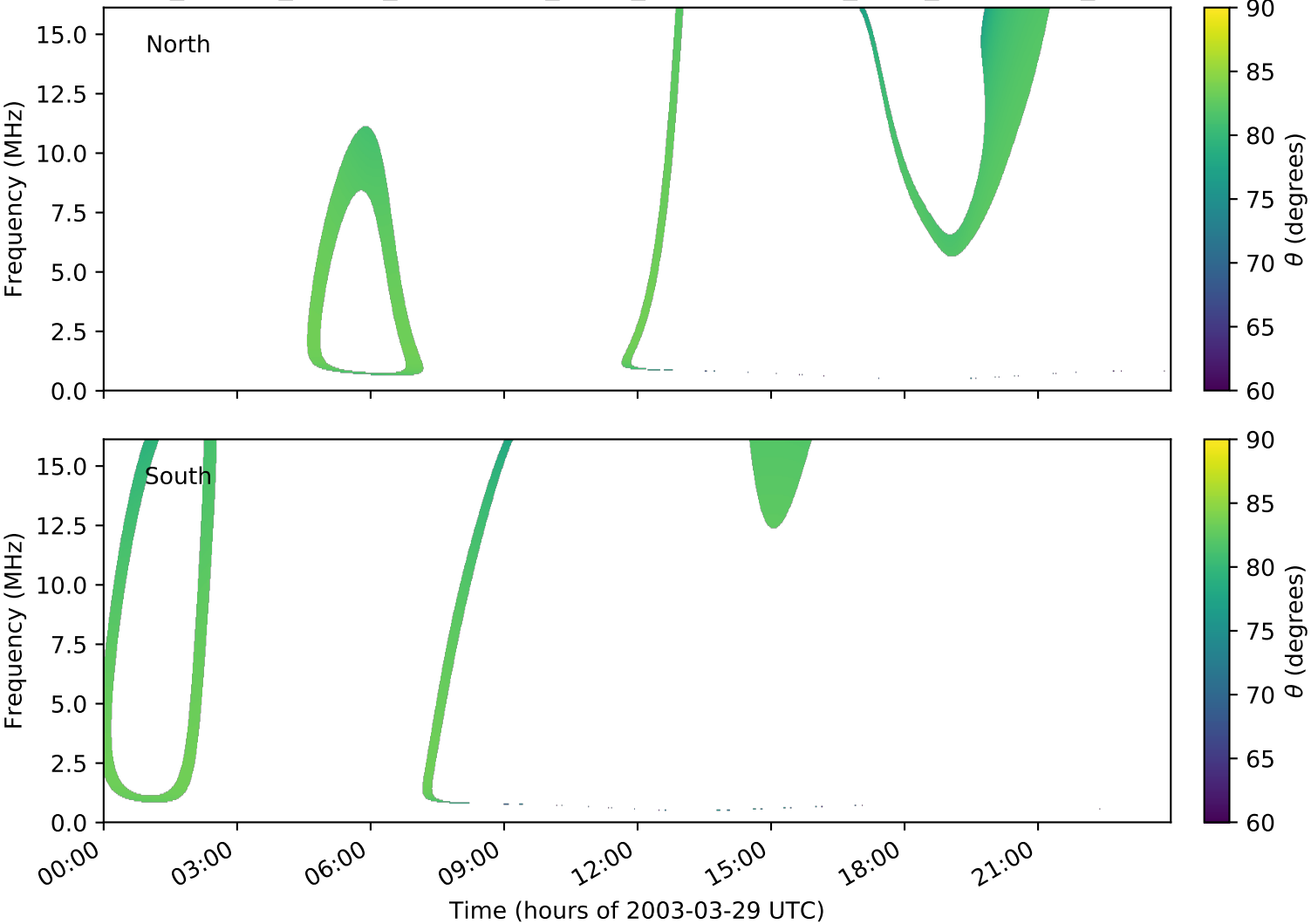
expres_cassini_jupiter_ganymede_isaac_lossc-wid1deg_3kev_20030329_v01.cdf
