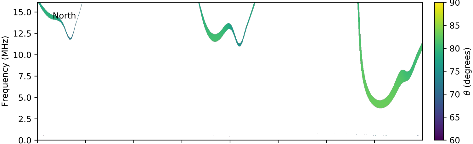
expres_cassini_jupiter_ganymede_isaac_lossc-wid1deg_3kev_20030324_v01.cdf
