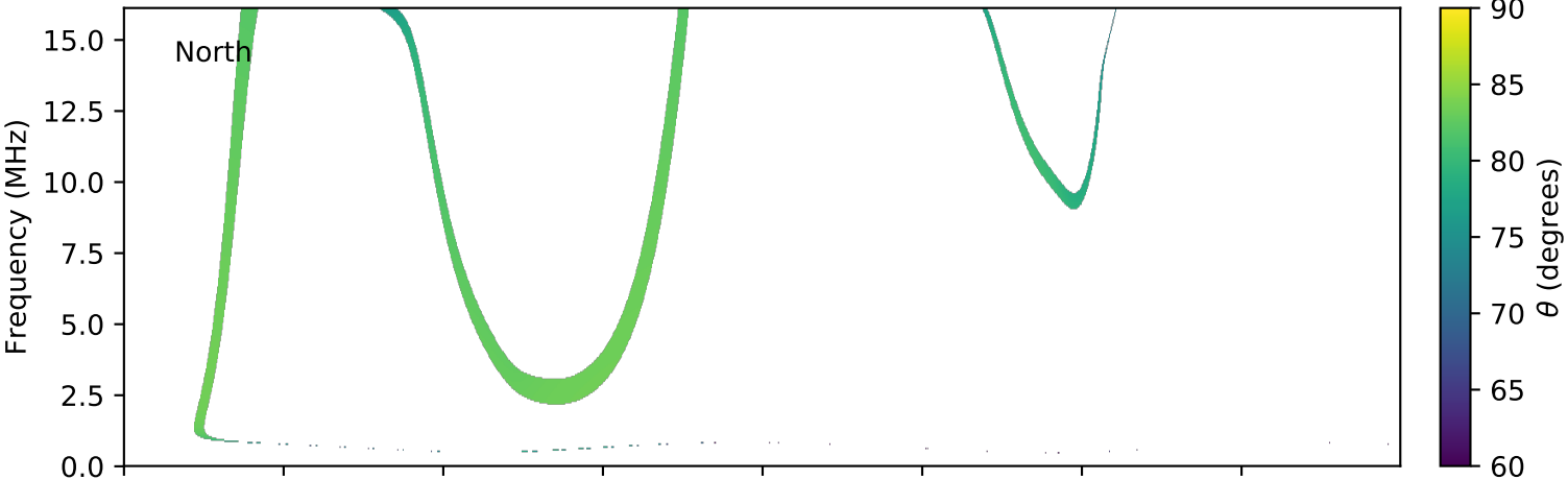
expres_cassini_jupiter_ganymede_isaac_lossc-wid1deg_3kev_20030315_v01.cdf
