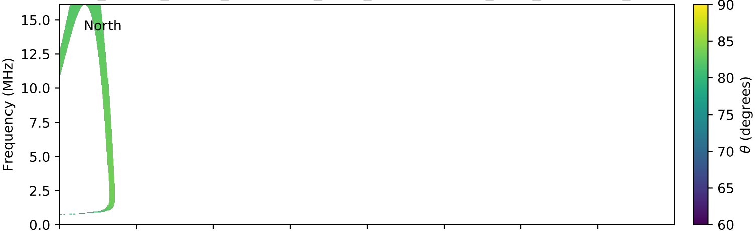
expres_cassini_jupiter_ganymede_isaac_lossc-wid1deg_3kev_20030311_v01.cdf
