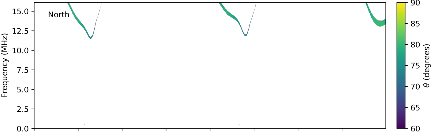
expres_cassini_jupiter_ganymede_isaac_lossc-wid1deg_3kev_20030309_v01.cdf
