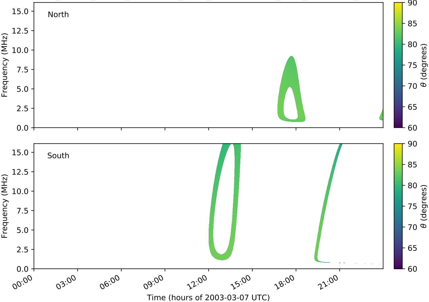
expres_cassini_jupiter_ganymede_isaac_lossc-wid1deg_3kev_20030307_v01.cdf
