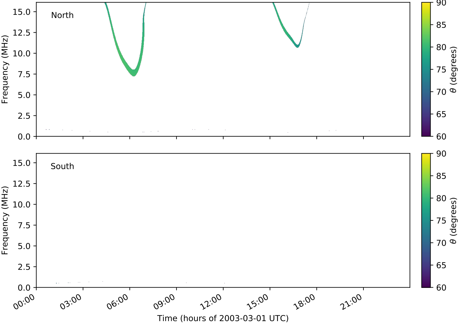
expres_cassini_jupiter_ganymede_isaac_lossc-wid1deg_3kev_20030301_v01.cdf
