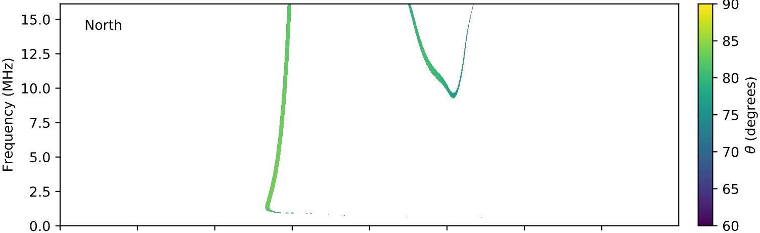
expres_cassini_jupiter_europa_isaac_lossc-wid1deg_3kev_20030330_v01.cdf
