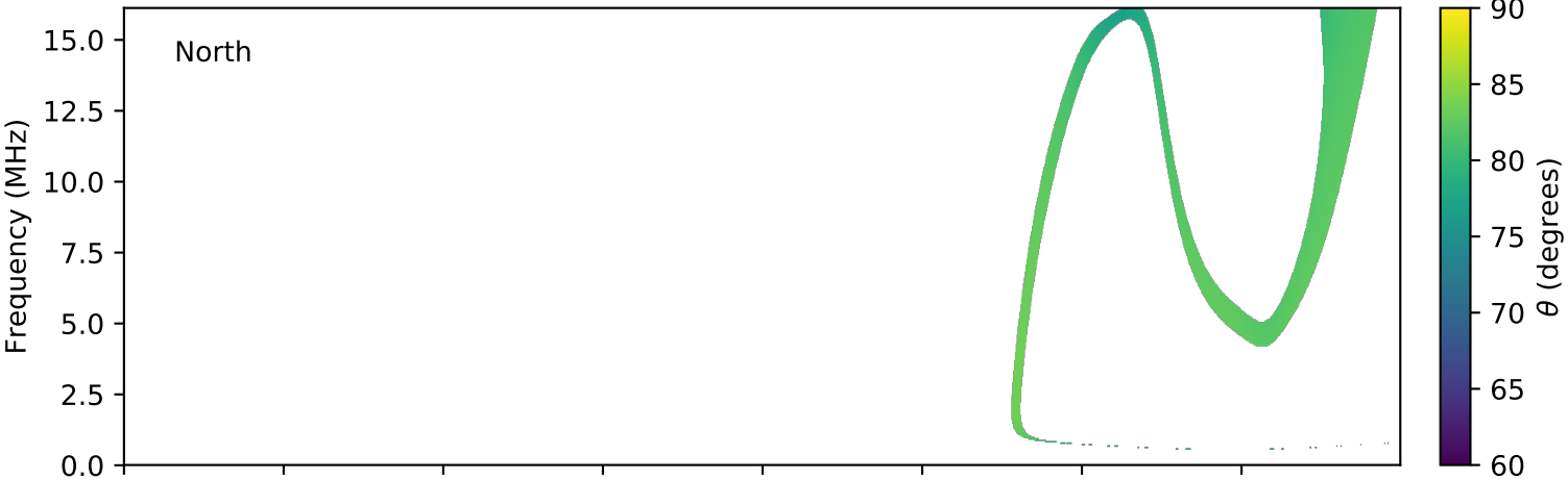
expres_cassini_jupiter_europa_isaac_lossc-wid1deg_3kev_20030326_v01.cdf
