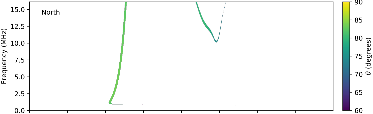
expres_cassini_jupiter_europa_isaac_lossc-wid1deg_3kev_20030323_v01.cdf
