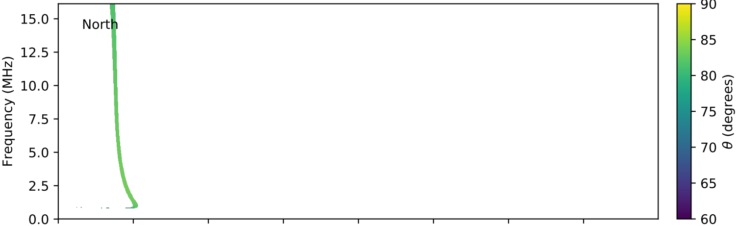
expres_cassini_jupiter_europa_isaac_lossc-wid1deg_3kev_20030321_v01.cdf
