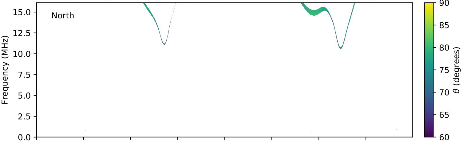
expres_cassini_jupiter_europa_isaac_lossc-wid1deg_3kev_20030320_v01.cdf
