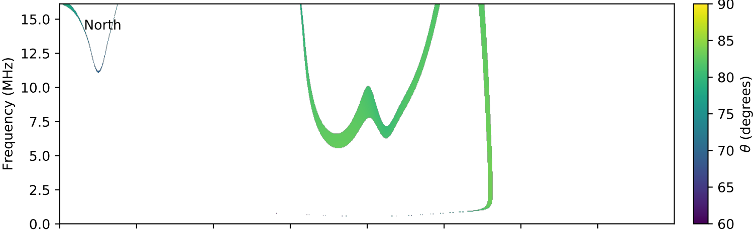
expres_cassini_jupiter_europa_isaac_lossc-wid1deg_3kev_20030317_v01.cdf
