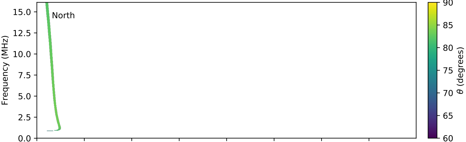
expres_cassini_jupiter_europa_isaac_lossc-wid1deg_3kev_20030314_v01.cdf
