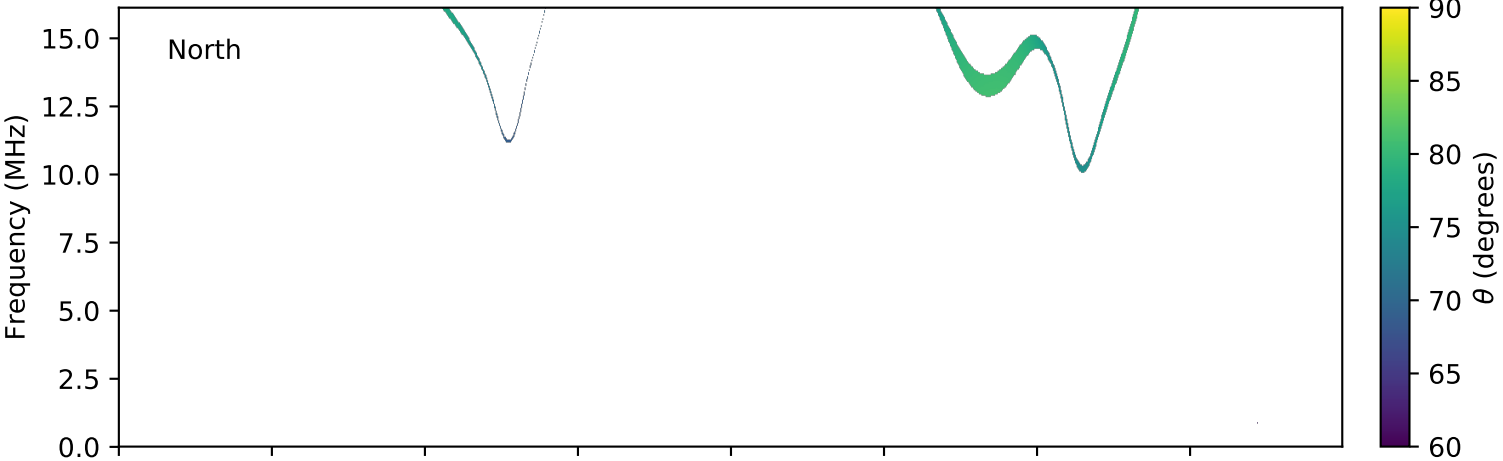
expres_cassini_jupiter_europa_isaac_lossc-wid1deg_3kev_20030313_v01.cdf
