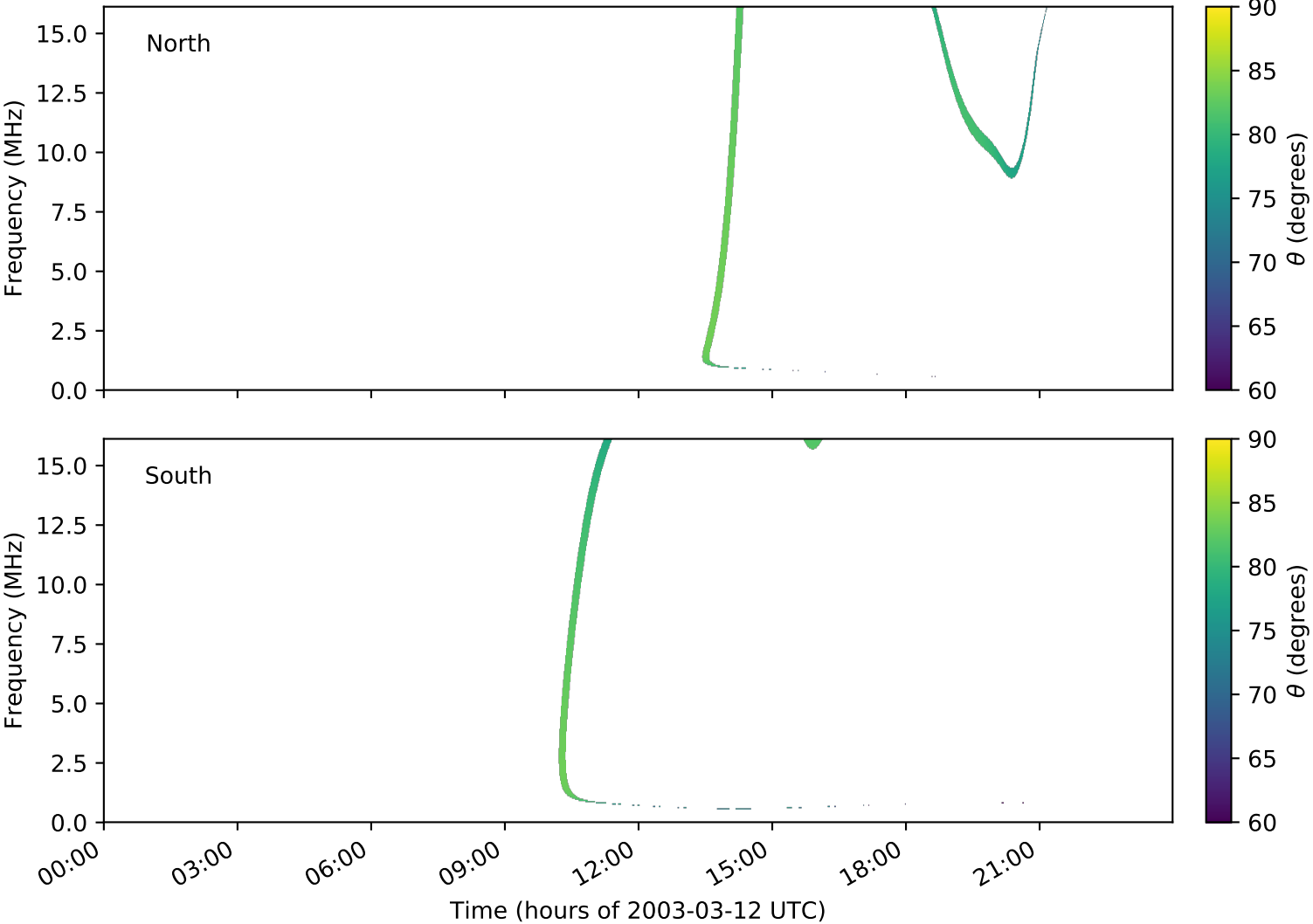
expres_cassini_jupiter_europa_isaac_lossc-wid1deg_3kev_20030312_v01.cdf
