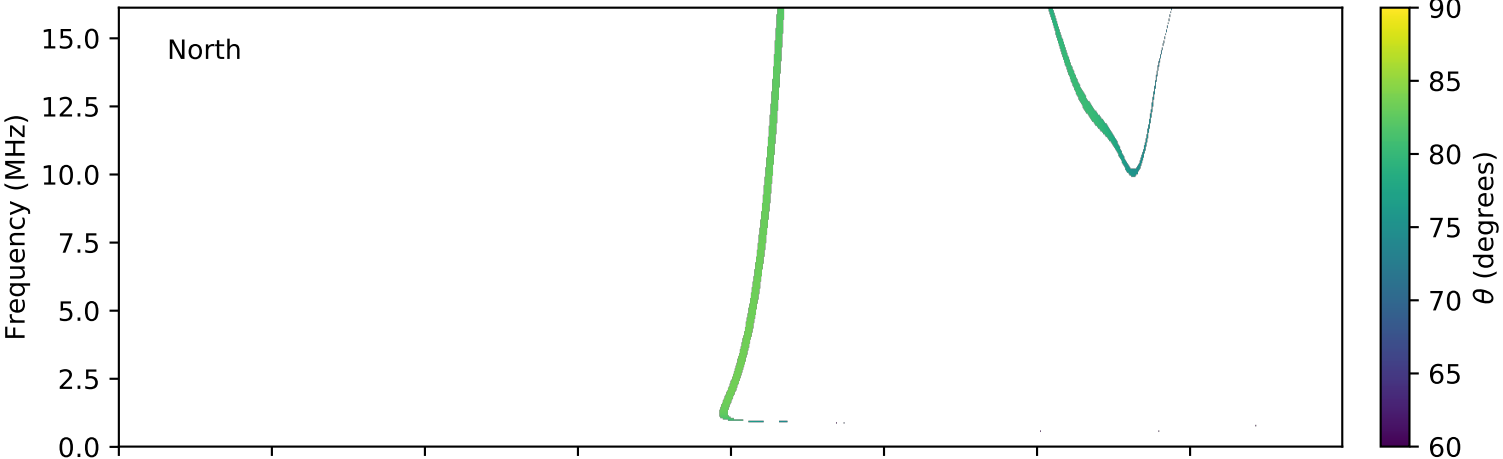
expres_cassini_jupiter_europa_isaac_lossc-wid1deg_3kev_20030305_v01.cdf
