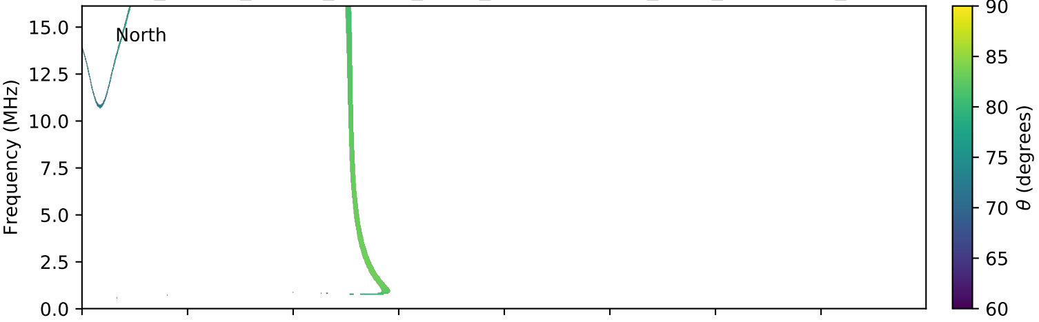
expres_cassini_jupiter_europa_isaac_lossc-wid1deg_3kev_20030303_v01.cdf
