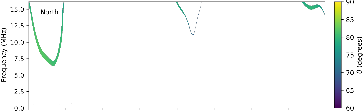
expres_cassini_jupiter_europa_isaac_lossc-wid1deg_3kev_20030302_v01.cdf
