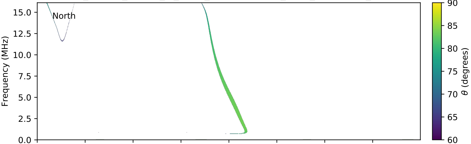
expres_cassini_jupiter_io_isaac_lossc-wid1deg_3kev_20030228_v01.cdf
