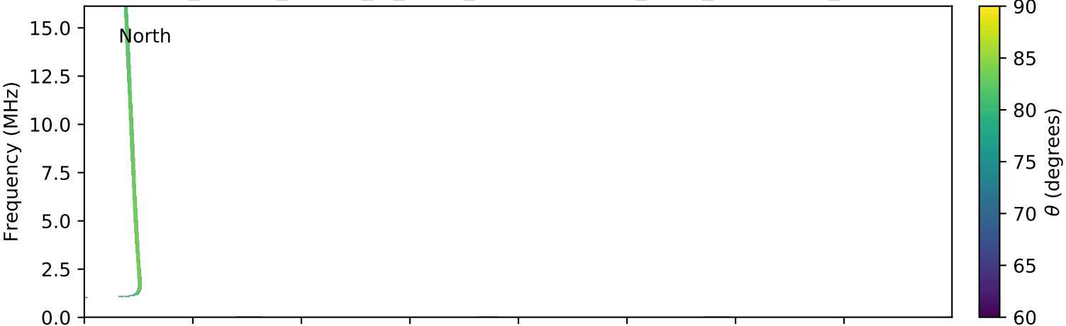
expres_cassini_jupiter_io_isaac_lossc-wid1deg_3kev_20030225_v01.cdf
