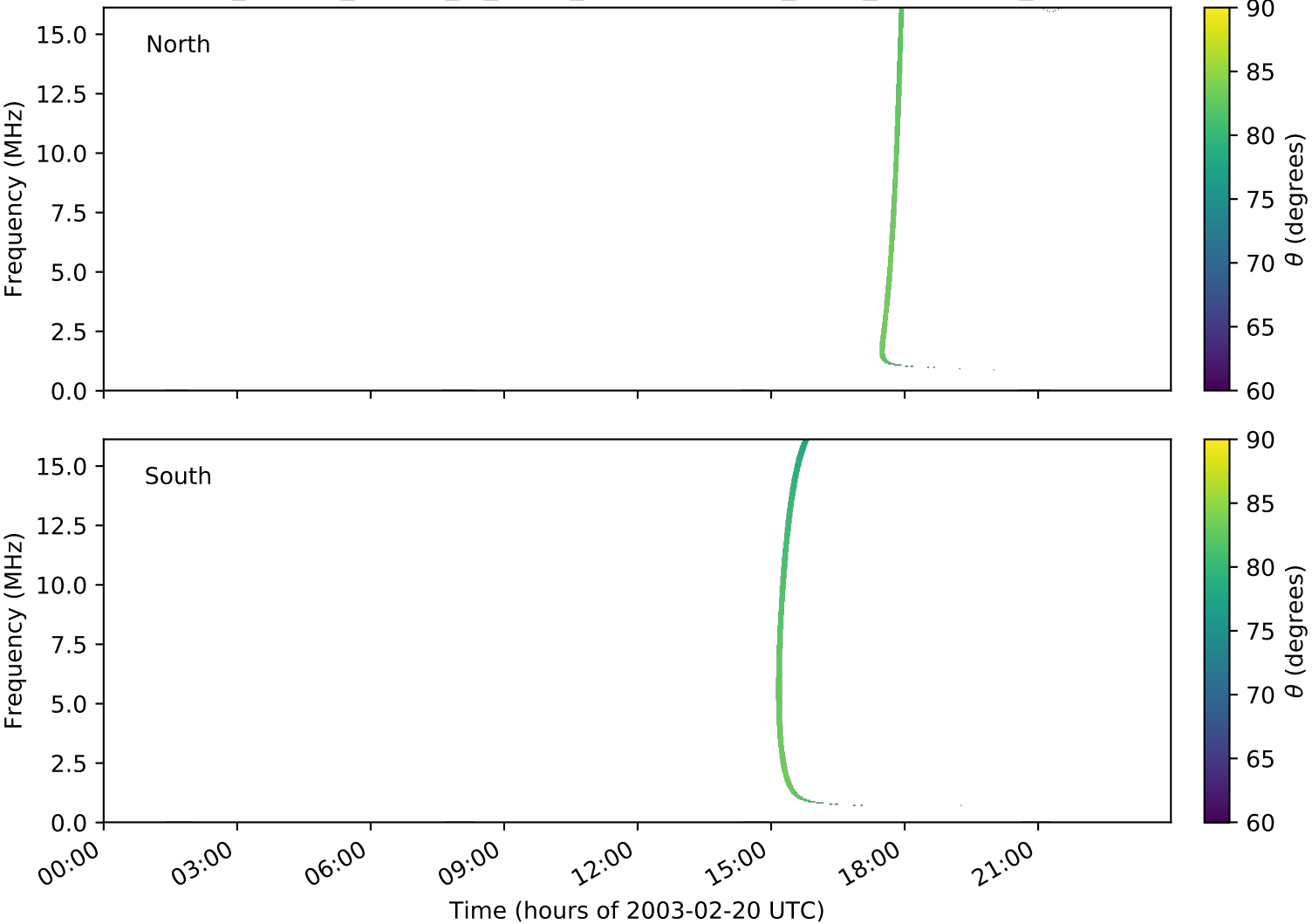
expres_cassini_jupiter_io_isaac_lossc-wid1deg_3kev_20030220_v01.cdf
