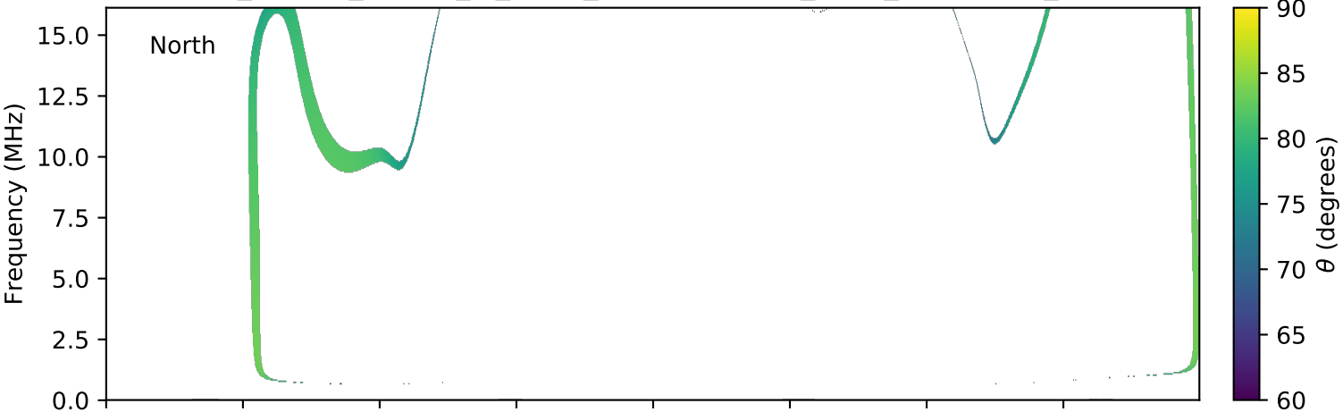
expres_cassini_jupiter_io_isaac_lossc-wid1deg_3kev_20030217_v01.cdf
