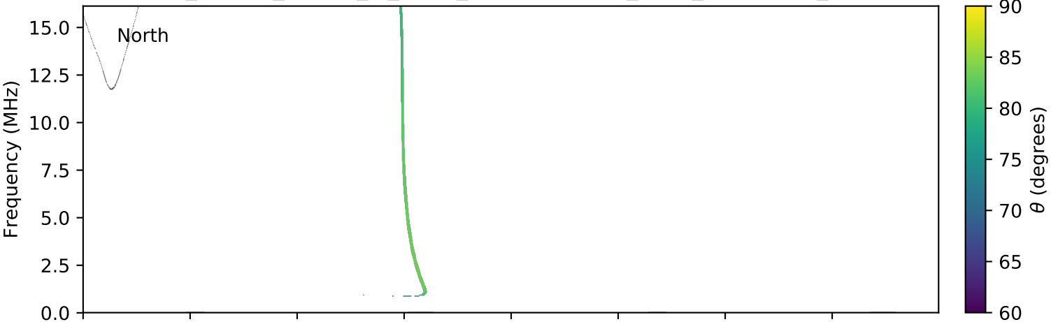
expres_cassini_jupiter_io_isaac_lossc-wid1deg_3kev_20030214_v01.cdf
