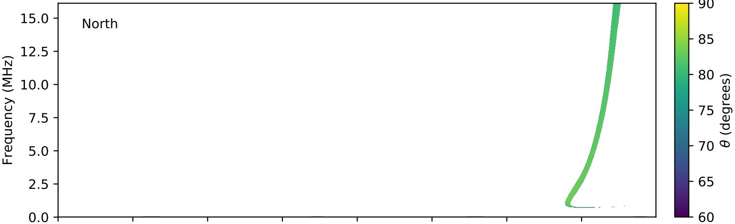
expres_cassini_jupiter_io_isaac_lossc-wid1deg_3kev_20030211_v01.cdf
