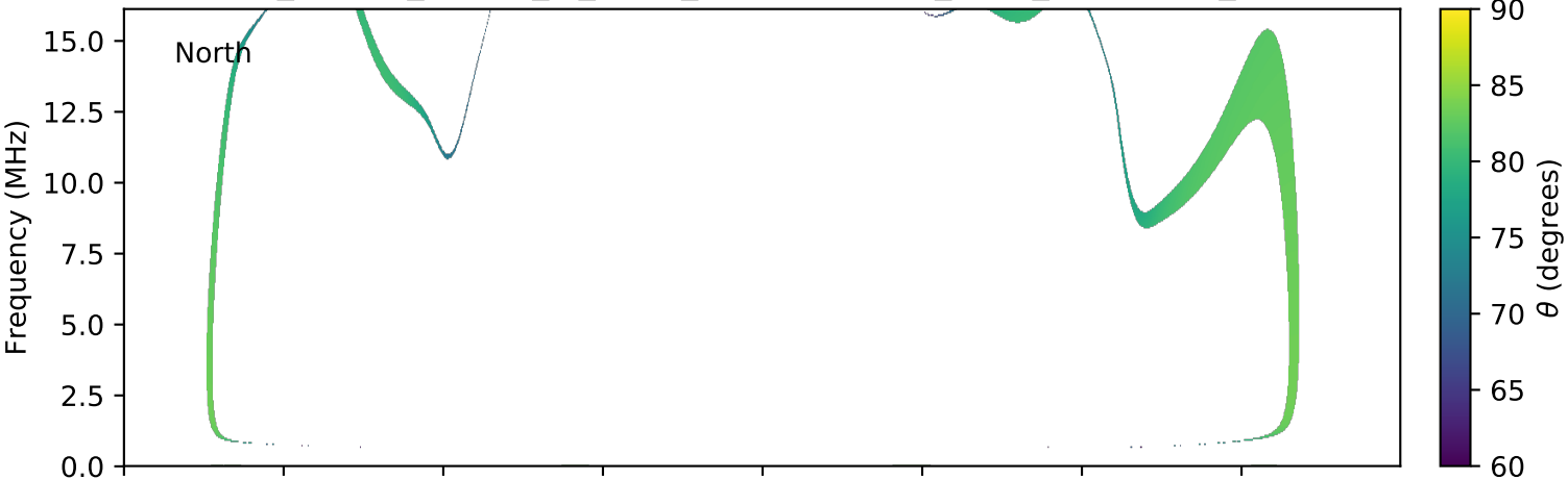
expres_cassini_jupiter_io_isaac_lossc-wid1deg_3kev_20030210_v01.cdf
