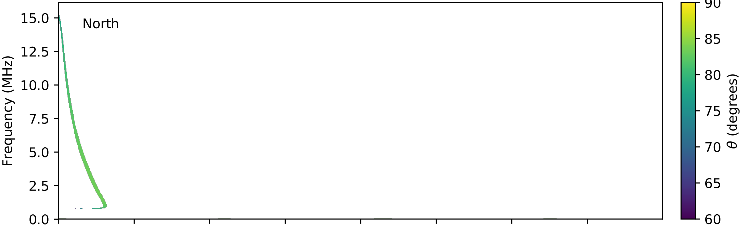
expres_cassini_jupiter_io_isaac_lossc-wid1deg_3kev_20030209_v01.cdf
