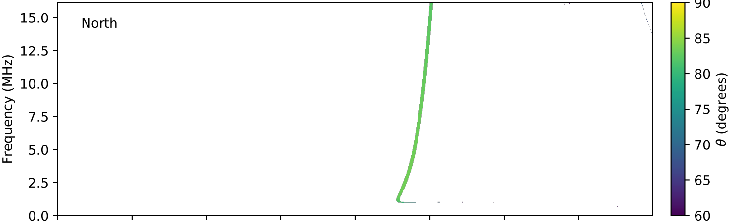
expres_cassini_jupiter_io_isaac_lossc-wid1deg_3kev_20030206_v01.cdf
