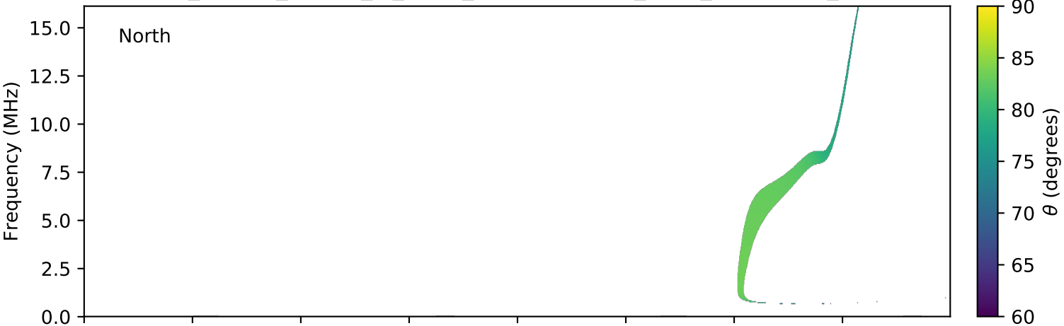
expres_cassini_jupiter_io_isaac_lossc-wid1deg_3kev_20030204_v01.cdf
