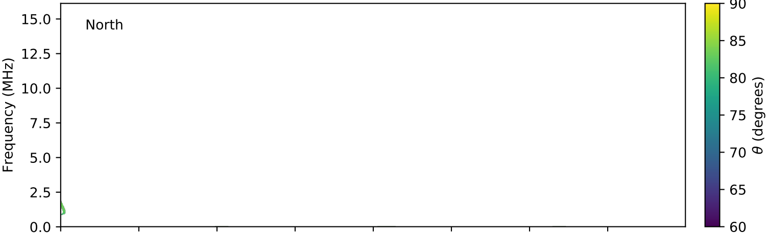
expres_cassini_jupiter_io_isaac_lossc-wid1deg_3kev_20030202_v01.cdf
