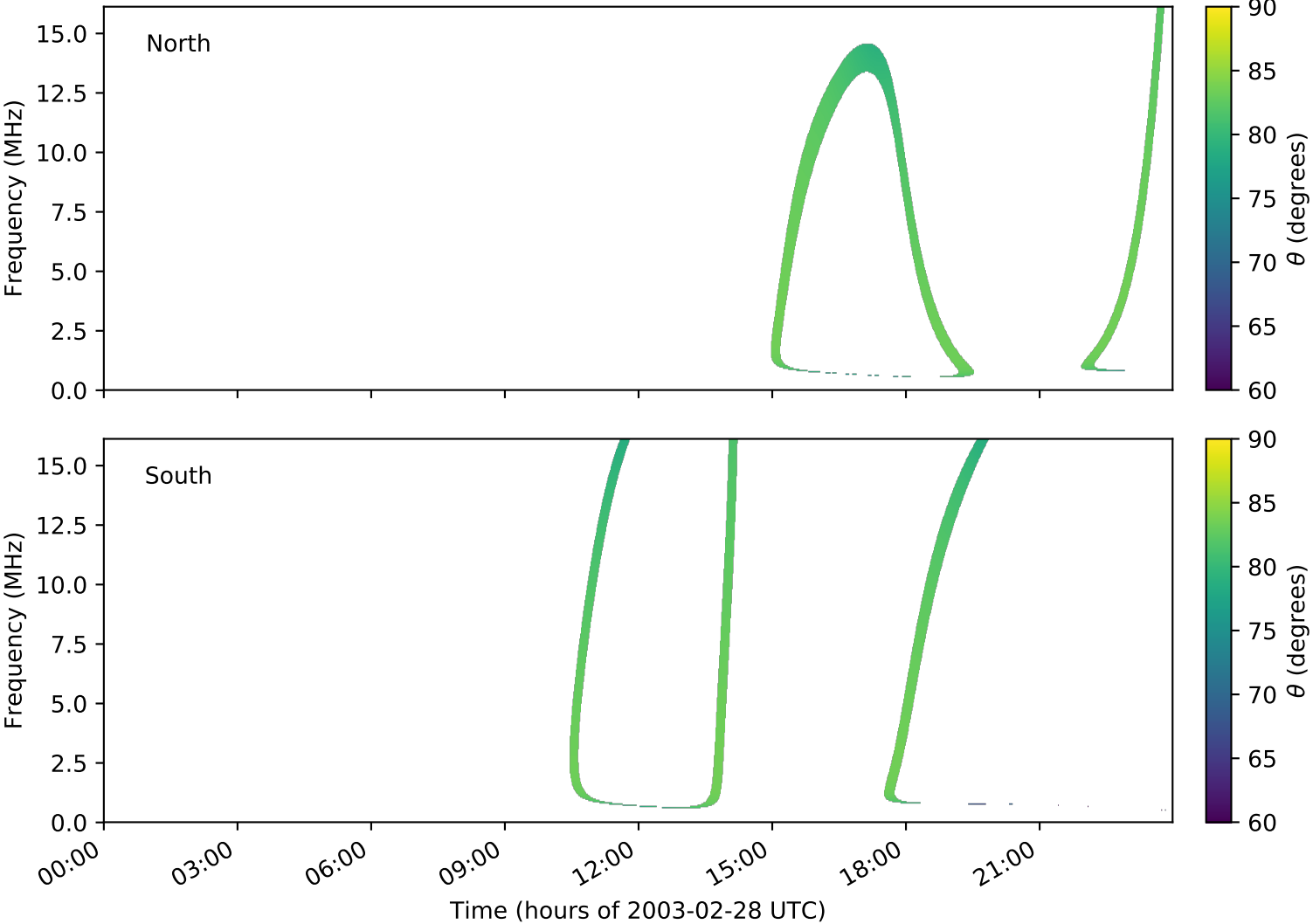
expres_cassini_jupiter_ganymede_isaac_lossc-wid1deg_3kev_20030228_v01.cdf
