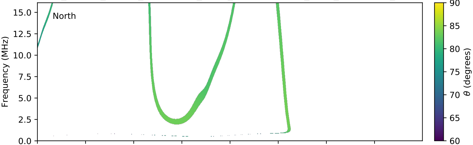
expres_cassini_jupiter_ganymede_isaac_lossc-wid1deg_3kev_20030224_v01.cdf
