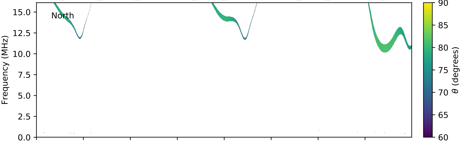
expres_cassini_jupiter_ganymede_isaac_lossc-wid1deg_3kev_20030223_v01.cdf
