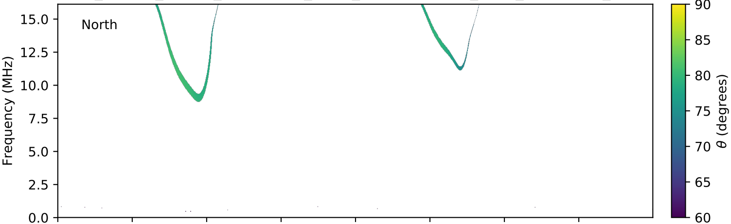
expres_cassini_jupiter_ganymede_isaac_lossc-wid1deg_3kev_20030222_v01.cdf
