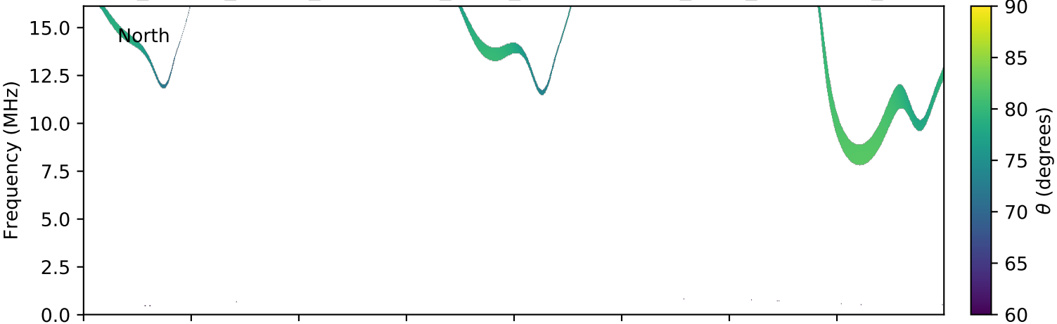
expres_cassini_jupiter_ganymede_isaac_lossc-wid1deg_3kev_20030216_v01.cdf
