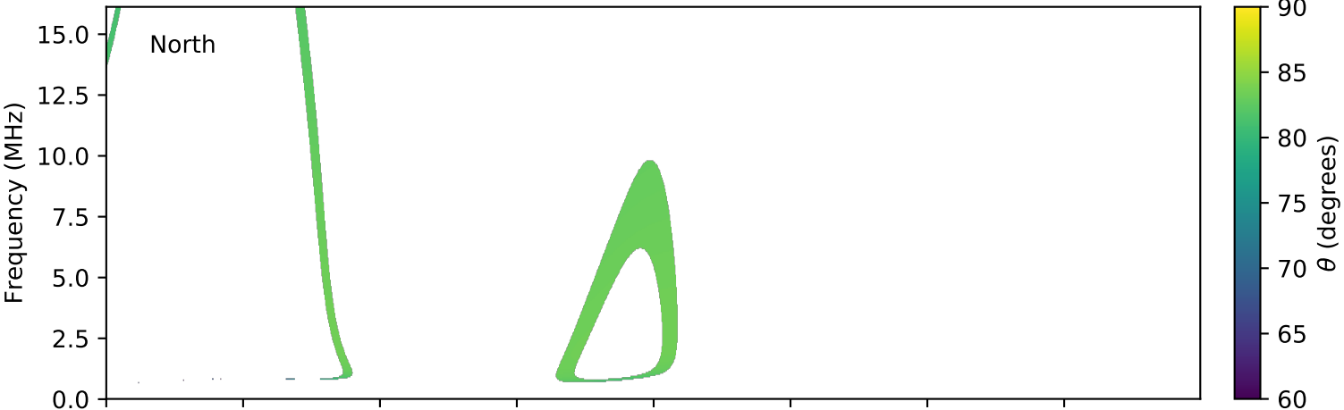
expres_cassini_jupiter_ganymede_isaac_lossc-wid1deg_3kev_20030210_v01.cdf
