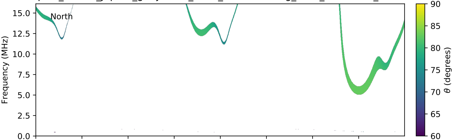
expres_cassini_jupiter_ganymede_isaac_lossc-wid1deg_3kev_20030209_v01.cdf
