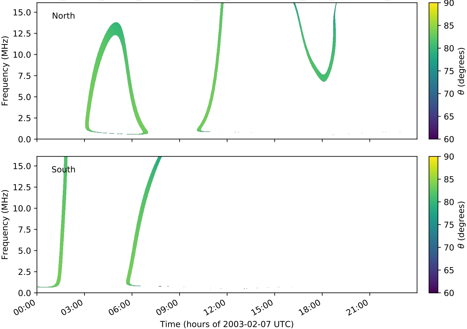
expres_cassini_jupiter_ganymede_isaac_lossc-wid1deg_3kev_20030207_v01.cdf
