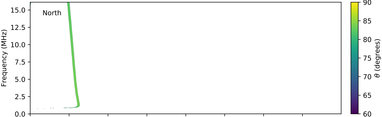
expres_cassini_jupiter_ganymede_isaac_lossc-wid1deg_3kev_20030203_v01.cdf
