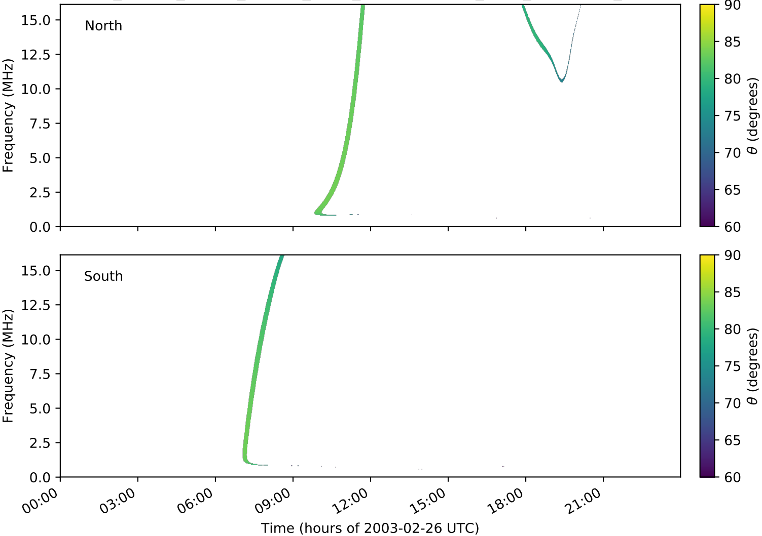
expres_cassini_jupiter_europa_isaac_lossc-wid1deg_3kev_20030226_v01.cdf
