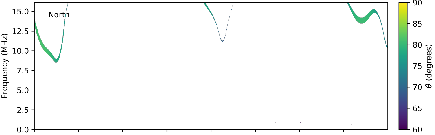
expres_cassini_jupiter_europa_isaac_lossc-wid1deg_3kev_20030223_v01.cdf
