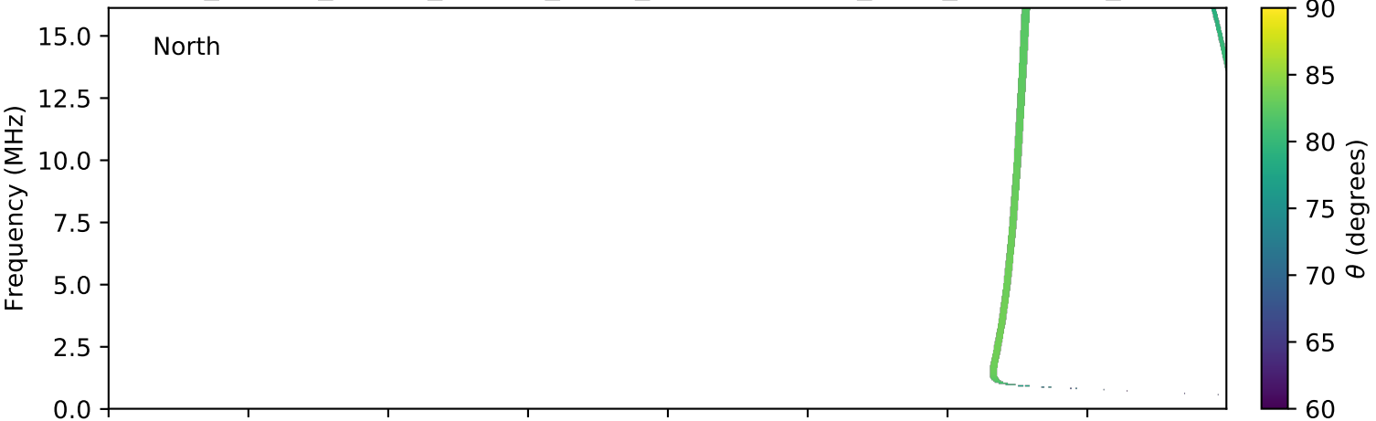
expres_cassini_jupiter_europa_isaac_lossc-wid1deg_3kev_20030222_v01.cdf
